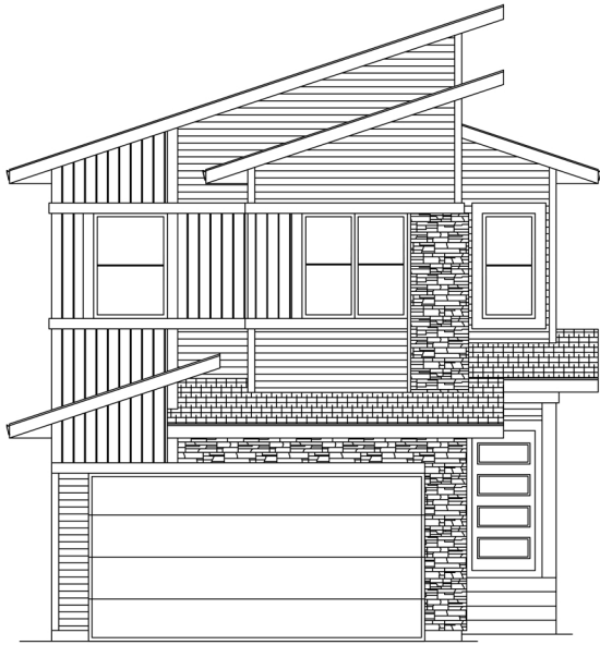
FRONT ELEVATION
